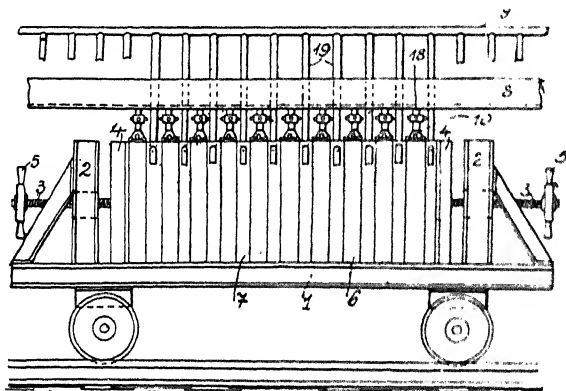
FIG. 20.—Holoubek's cooler.
