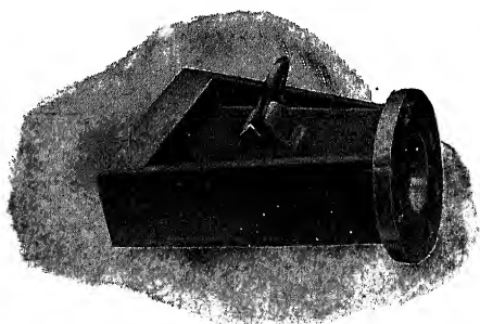
FIG. 1.—Skimmer, with flange for attachment to skimmer-pipe.
