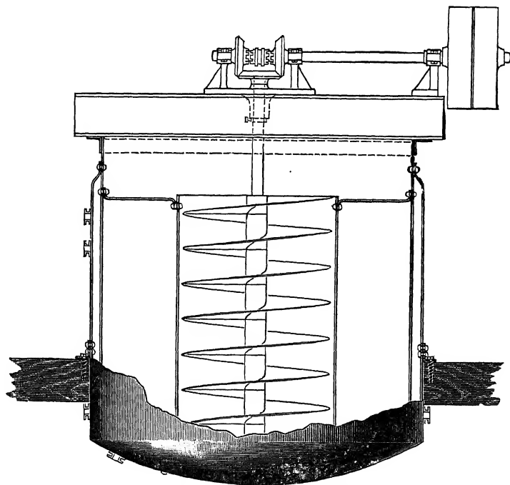
FIG. 7.—Mechanical crutcher.
