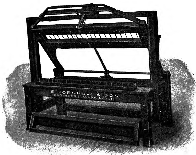
FIG. 12.—Barring machine.
